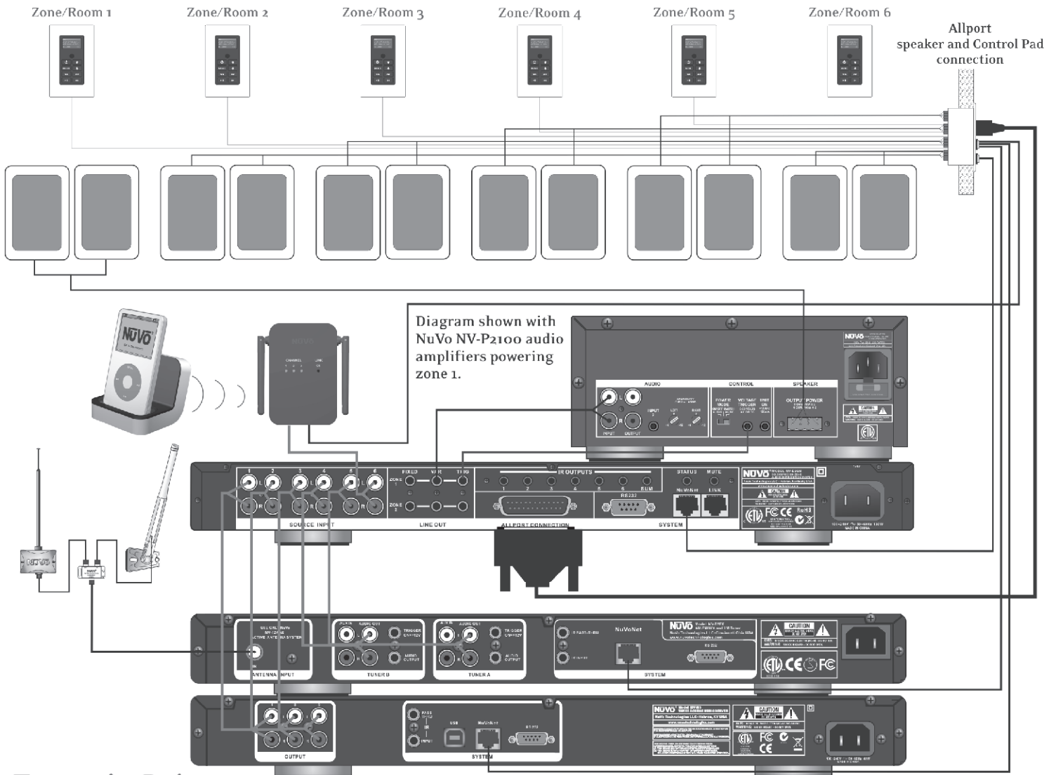
Essentia Suite Wiring Diagram
