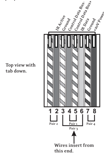
Fig. 1: EIA 568A and 568B wiring scheme for CAT5 Cable
